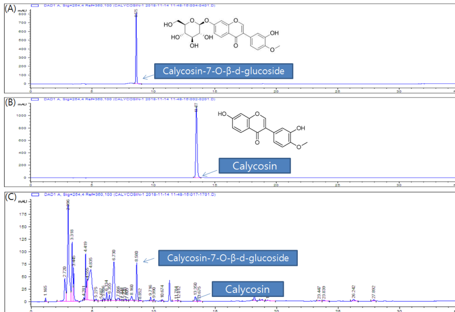
Fig. 1. Selected chromatogram of calycosin-7-O-β-D-glucoside (A) calycosin (B) and sample (C) from A. membranaceus .
